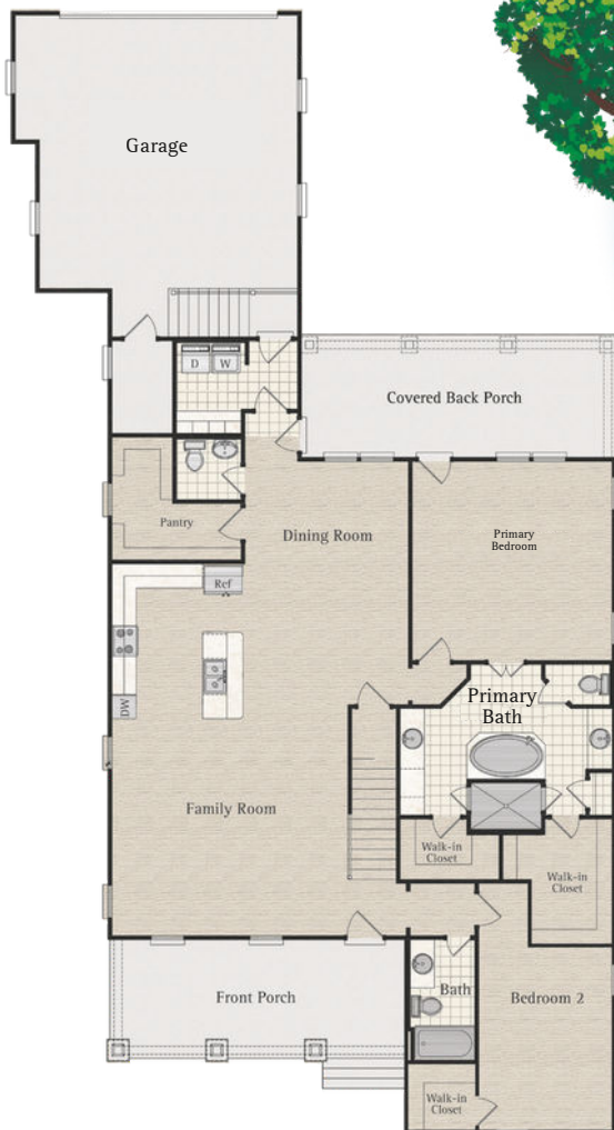
1st Floor
