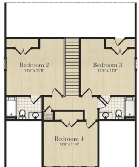
2nd Floor
